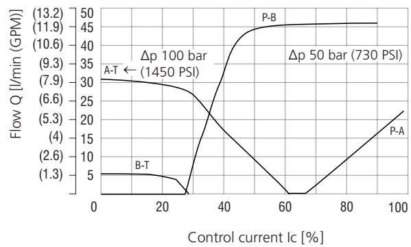
Operating limits SD2P-B4/H3Y13-25
