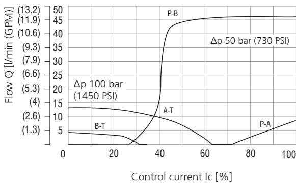
Operating limits SD2P-B4/H3Y13-5
